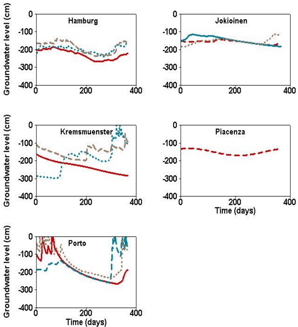
Figure 1 Examples of yearly fluctuations in groundwater level for FOCUS scenarios simulated with SWAP for PEARL. Heavily dashed lines are for average years, solid lines for dry years and lightly dashed lines for wet years. All simulations are for potatoes assuming no irrigation.
