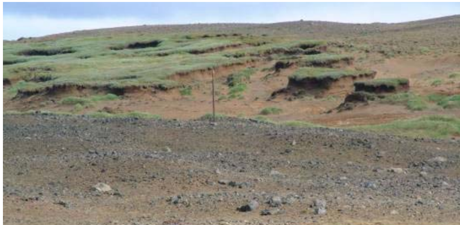
Figure 1. At rofabards (erosion escarpments), thick Andosols are removed by the forces of wind and water leaving shallow and poor soils with limited vegetation cover (note a telephone pole at the center of the image). The picture was taken in northeast Iceland in 2002.
